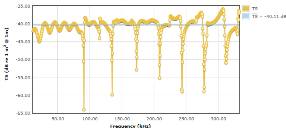
Figure 2.1. Theoretical target strength ( TS ; dB re 1 \text{ m}^2 at 1 \text{ m} ) values for a 38.1-mm-diameter sphere made from tungsten carbide with 6% cobalt (WC), at t_w = 13.5^\circ\text{C} , s = 33.3 \text{ psu} , pressure = 25.0 \text{ dbar} , c_w = 1500 \text{ m} \cdot \text{s}^{-1} , and \rho_w = 1025.0 \text{ kg} \cdot \text{m}^{-3} . The mean TS , \overline{TS} , is calculated in the linear domain, over the displayed bandwidth (12–333 kHz). This image is from http://swfscdata.nmfs.noaa.gov/AST/SphereTS/ , an application that implements the sphere TS model in MacLennan (1981).
