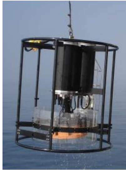
Figure 1.11. Cast echosounder systems are used to position echosounders and deep-water transducers closer to demersal fish targets. In this case, the transducer is gimballed to provide vertical measurements, irrespective of platform tilt due to, e.g. water current.
