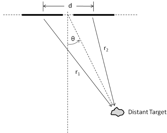
Figure 1.7. The geometry for a two-dimensional split-beam. The subarrays are represented as thick dark lines, separated by a distance d_{eff} ( d in the figure).
