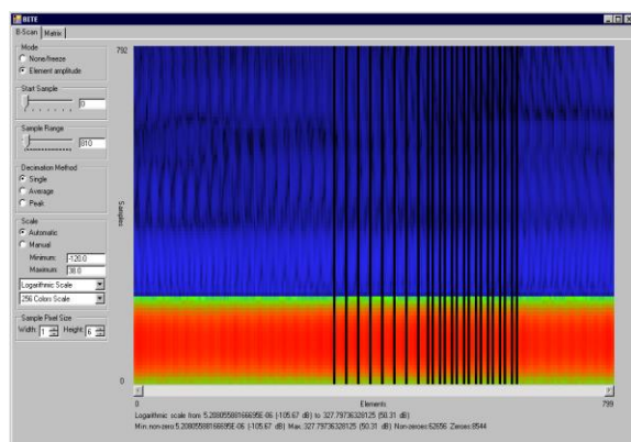
Figure. 4.8a. Matrix view during a reception period showing six disabled elements (black) and one defective, high-intensity element (red).
