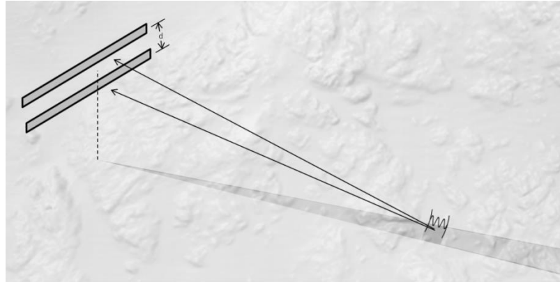
Figure 1.8. The geometry for bearing estimations using split-beam sidescan sonar. Two single-beam sidescan transducers, separated by a distance d_{eff} ( d in the figure), are used to measure electrical phase differences and thus estimate the bearing angles to the seabed.
