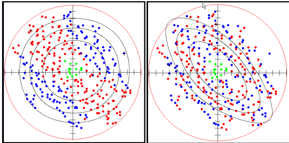
Figure 4.2. Example beam maps for a transducer with a disconnected upper-right quadrant. In this case, TS measurements could not be made towards the edges of the upper-right and lower-left quadrants. The beam model (left) has concentric lines, but banding in the positive (red) and negative residuals (blue) indicates a problem. The polynomial model (right) shows slanted ellipsoids with more randomly distributed residuals, also indicating a problem with the transducer or receiver.
