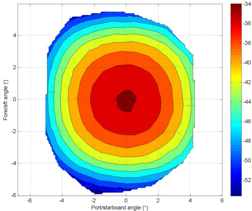
Figure 2.9. Example of the beam model for a 7°-beamwidth, 38-kHz transducer, estimated using TS measurements of a 60.0-mm diameter copper sphere. Indications of a good quality calibration are: uniform coverage of the sphere-TS measurements (+), and smooth, circular, and concentric contours. The colours indicate the observed (beam uncompensated) sphere TS (dB).
