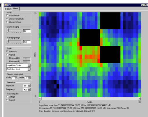
Figure. 4.8b. Matrix view during a transmission period showing three disabled elements (black) and one defective, high-intensity element (green amidst blue).
