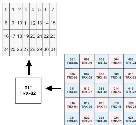
Figure 4.7. Each of 25 TRX32 cards, numbered 0–24 in the 5 × 5 matrix, control 32 of the 800 transducer elements.
